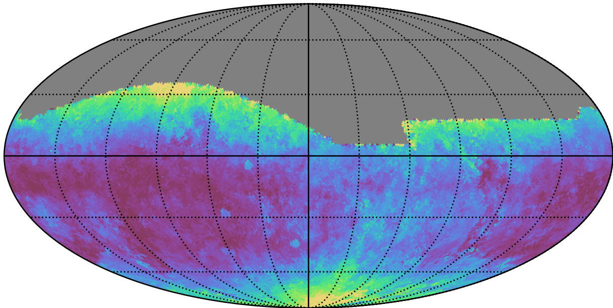
noroll_mjdp365_v3.4_10yrs All sky g band: Median seeingEff
