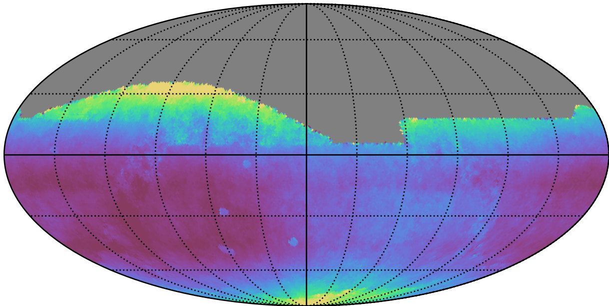
noroll_mjdp365_v3.4_10yrs All sky all bands: Median seeingEff
