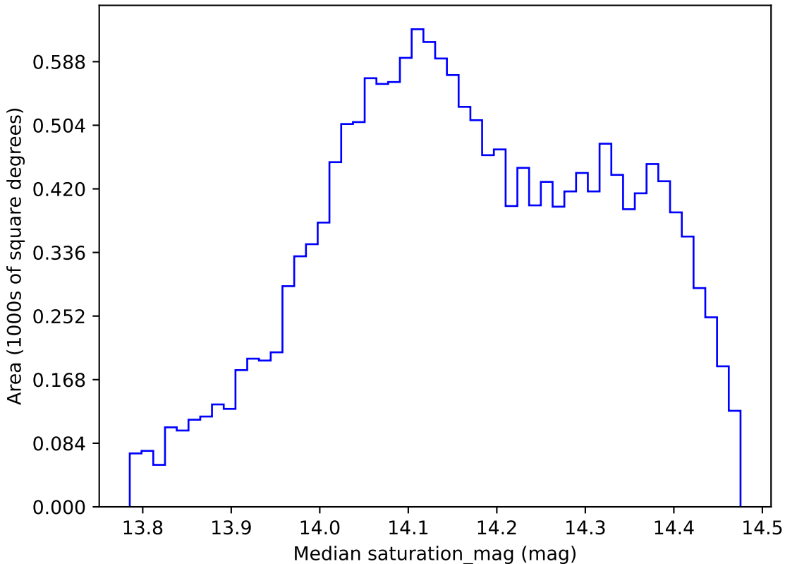
noroll_mjdp365_v3.4_10yrs WFD z band: Median saturation_mag
