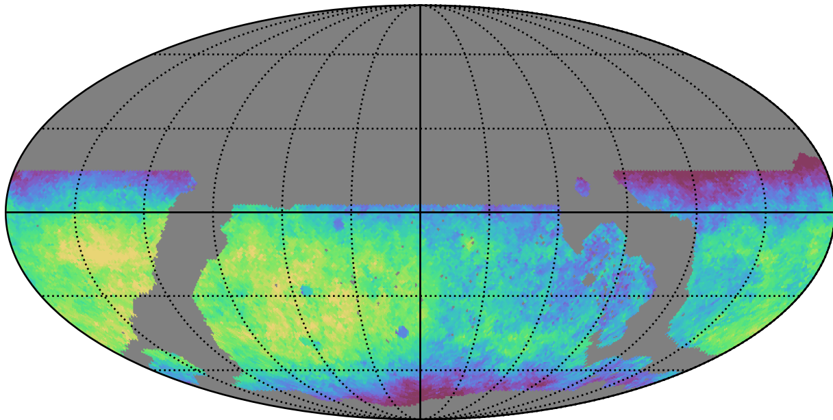
noroll_mjdp365_v3.4_10yrs WFD y band: Median saturation_mag
