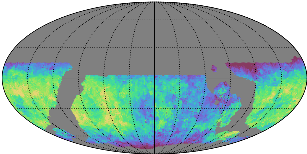
noroll_mjdp365_v3.4_10yrs WFD u band: Median saturation_mag
