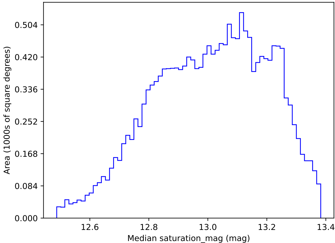
noroll_mjdp365_v3.4_10yrs WFD u band: Median saturation_mag
