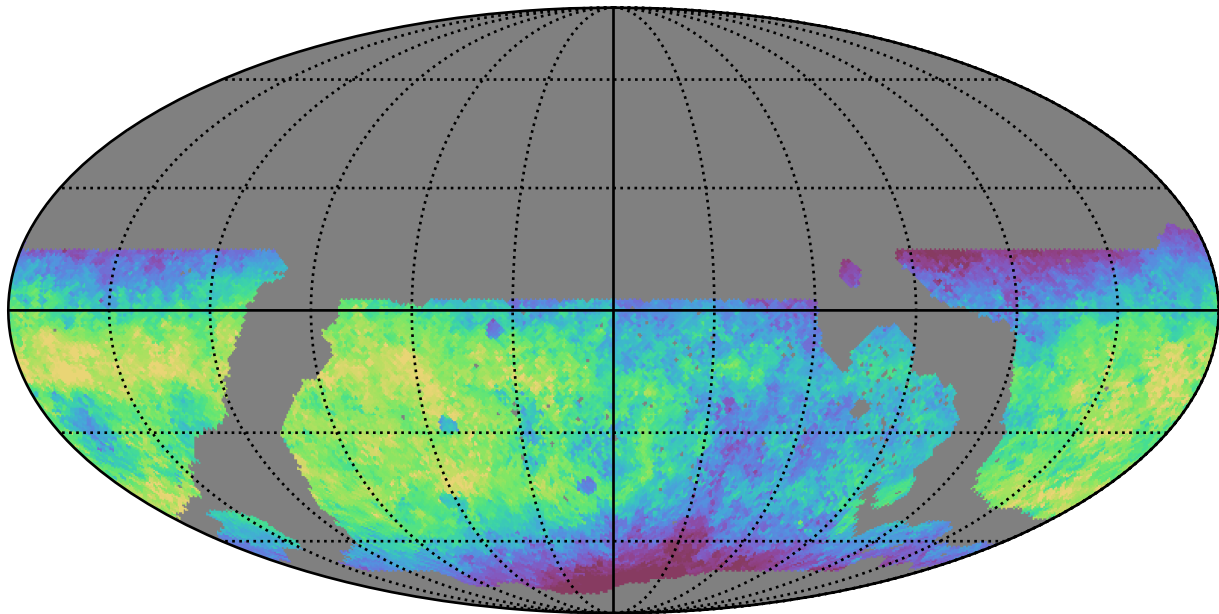
noroll_mjdp365_v3.4_10yrs WFD g band: Median saturation_mag
