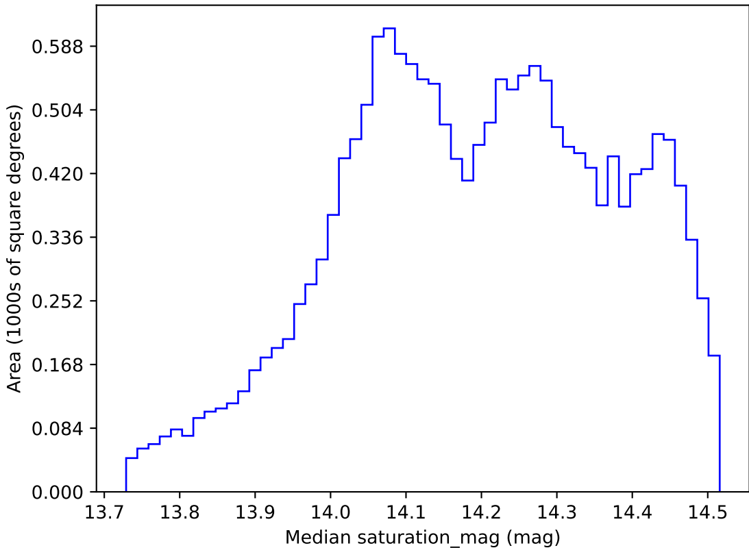
noroll_mjdp365_v3.4_10yrs WFD all bands: Median saturation_mag
