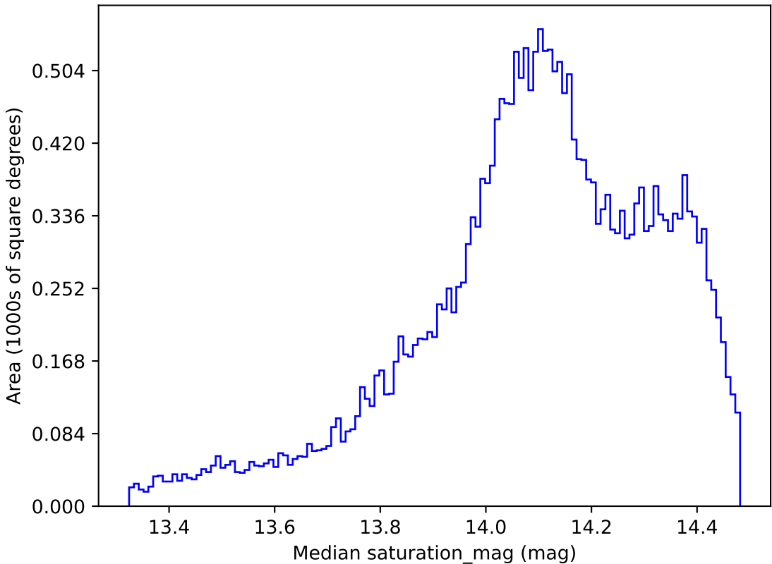
noroll_mjdp365_v3.4_10yrs All sky z band: Median saturation_mag
