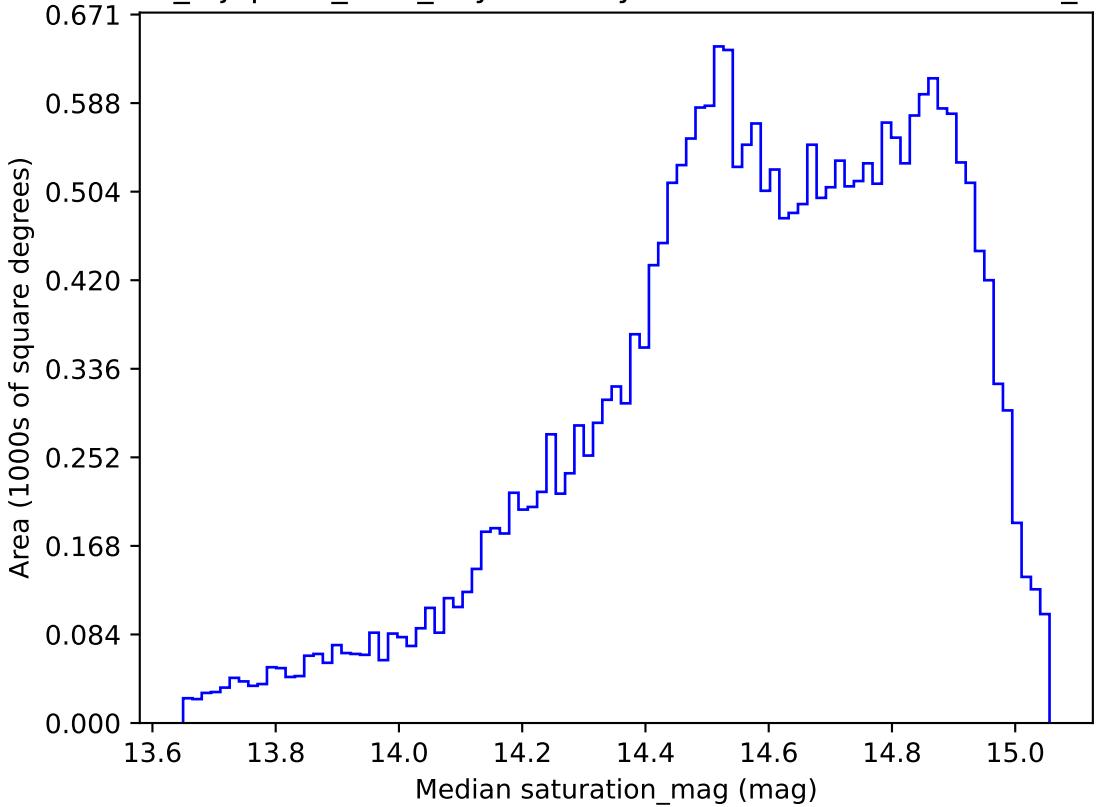
noroll_mjdp365_v3.4_10yrs All sky r band: Median saturation_mag
