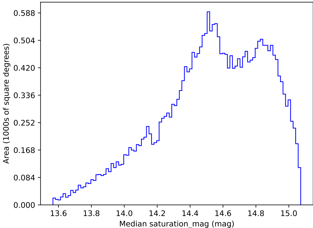
noroll_mjdp365_v3.4_10yrs All sky g band: Median saturation_mag
