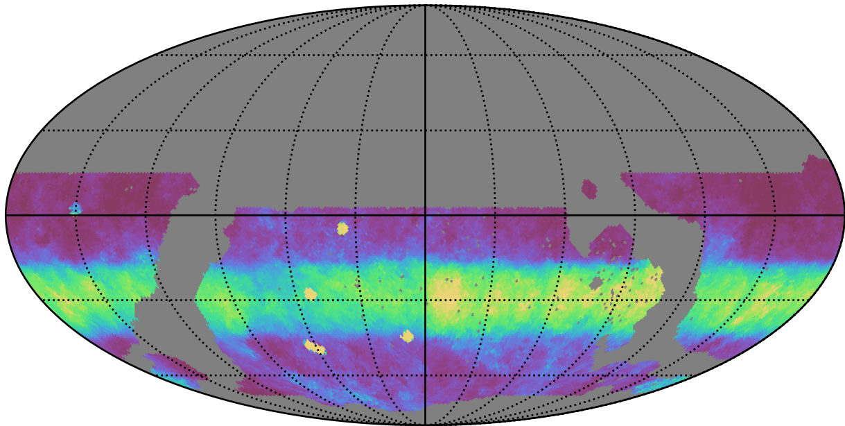
noroll_mjdp365_v3.4_10yrs WFD z band: Median normairmass
