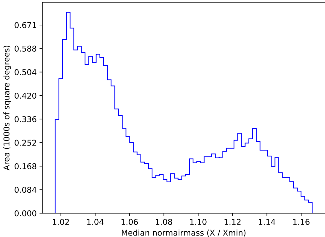
noroll_mjdp365_v3.4_10yrs WFD z band: Median normairmass
