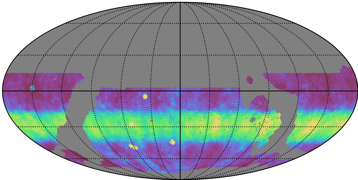
noroll_mjdp365_v3.4_10yrs WFD y band: Median normairmass
