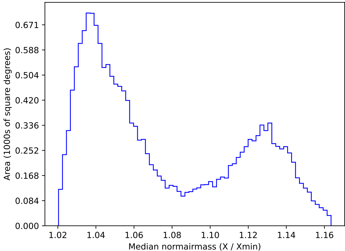
noroll_mjdp365_v3.4_10yrs WFD y band: Median normairmass
