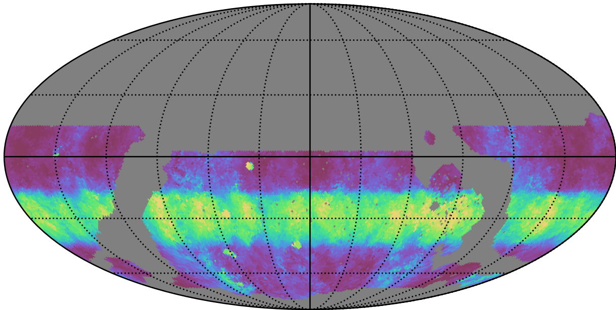
noroll_mjdp365_v3.4_10yrs WFD u band: Median normairmass
