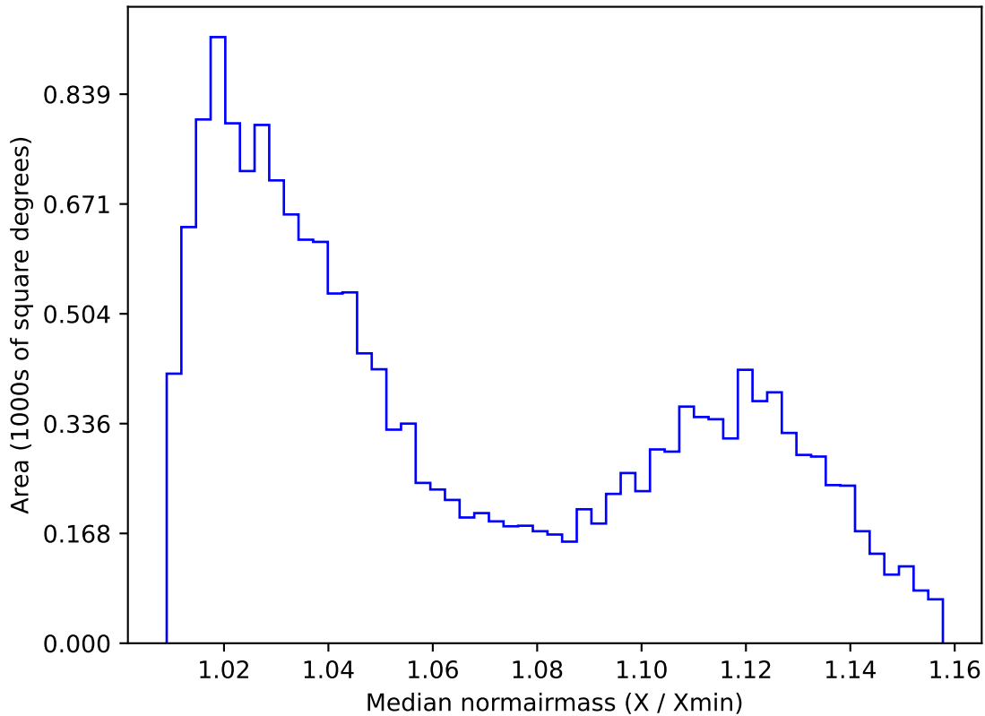
noroll_mjdp365_v3.4_10yrs WFD u band: Median normairmass
