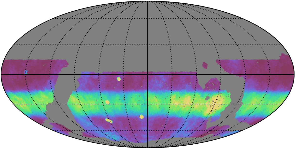
noroll_mjdp365_v3.4_10yrs WFD r band: Median normairmass
