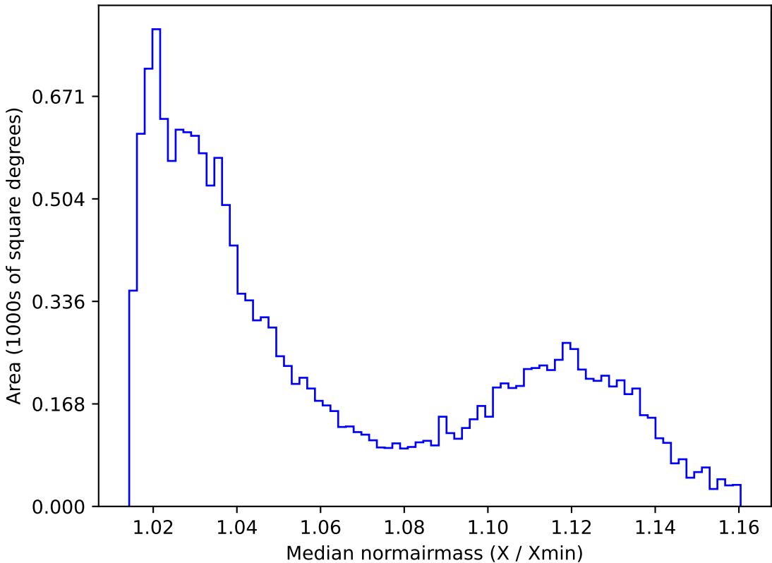
noroll_mjdp365_v3.4_10yrs WFD r band: Median normairmass
