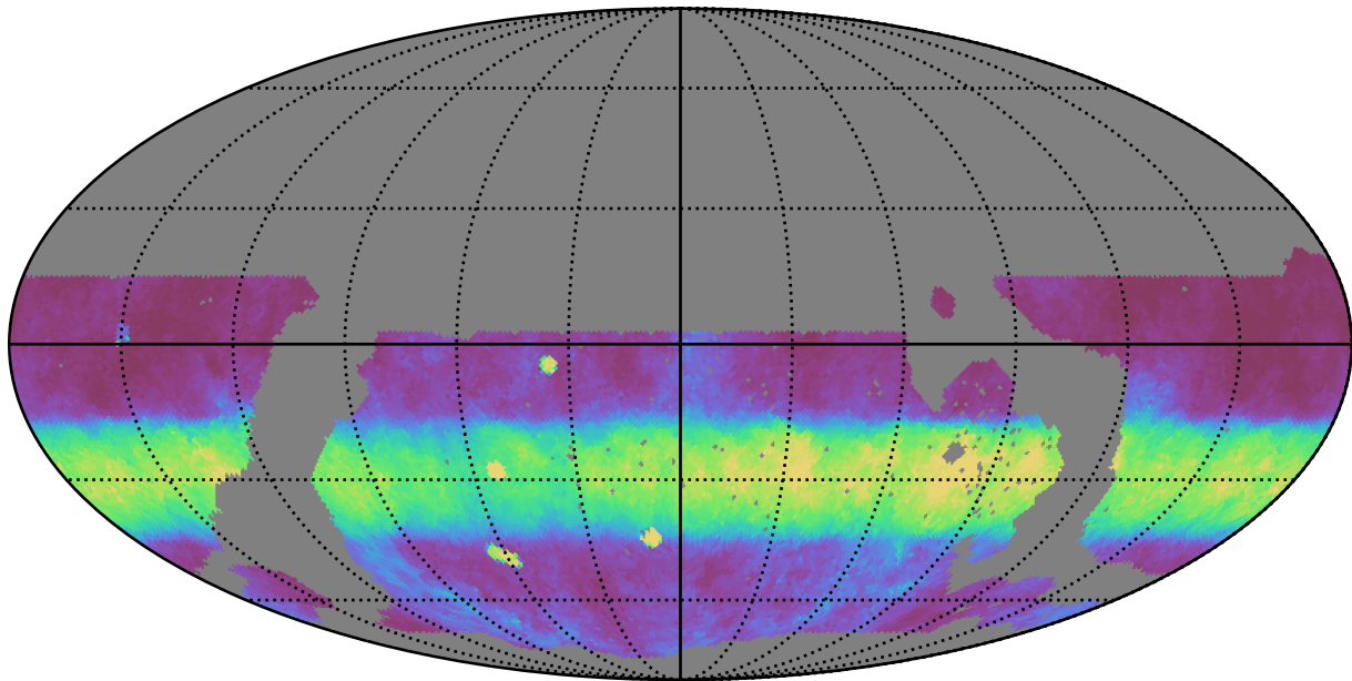
noroll_mjdp365_v3.4_10yrs WFD i band: Median normairmass
