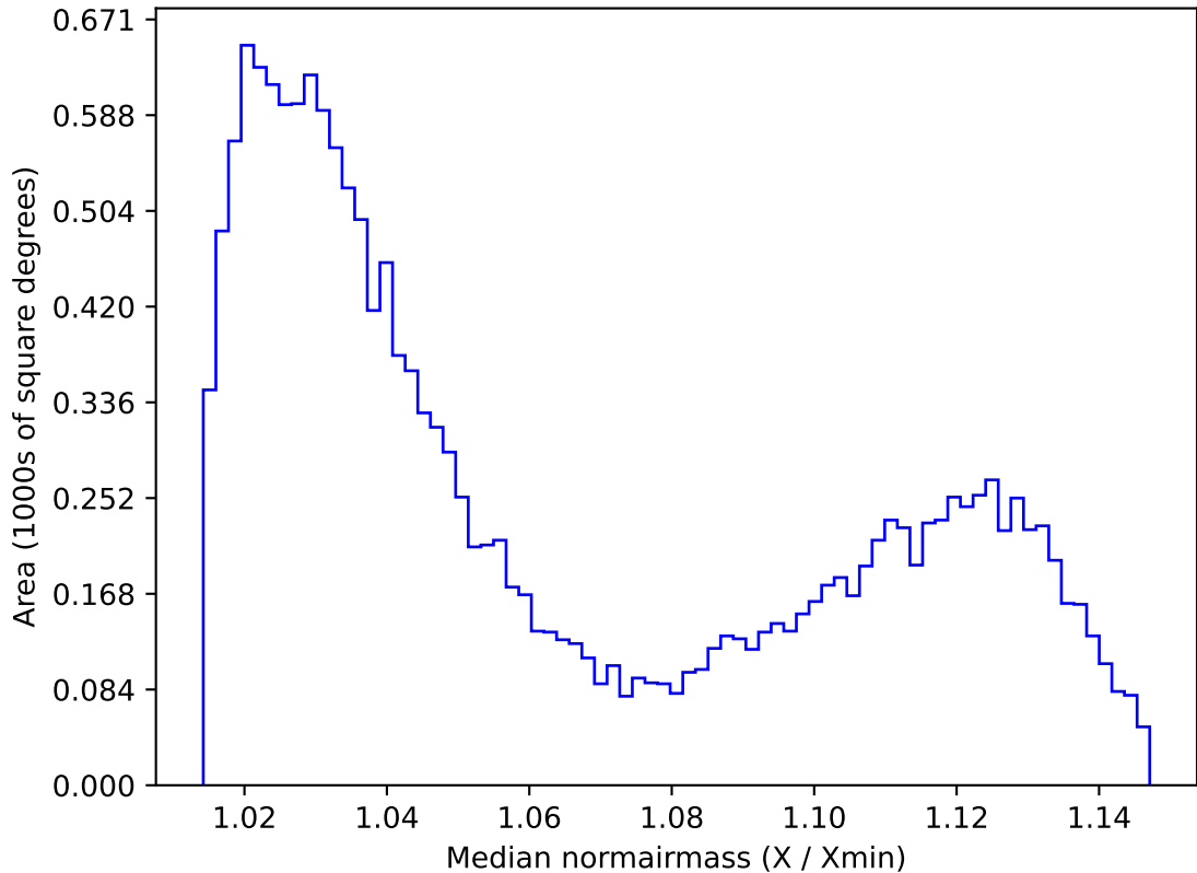
noroll_mjdp365_v3.4_10yrs WFD i band: Median normairmass
