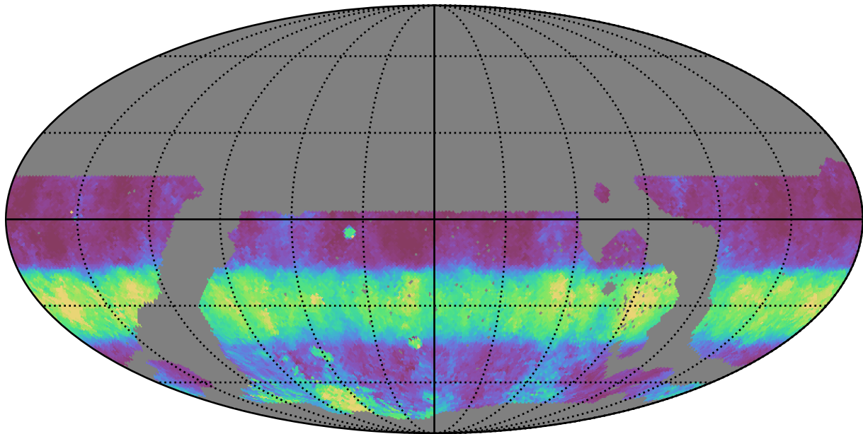
noroll_mjdp365_v3.4_10yrs WFD g band: Median normairmass
