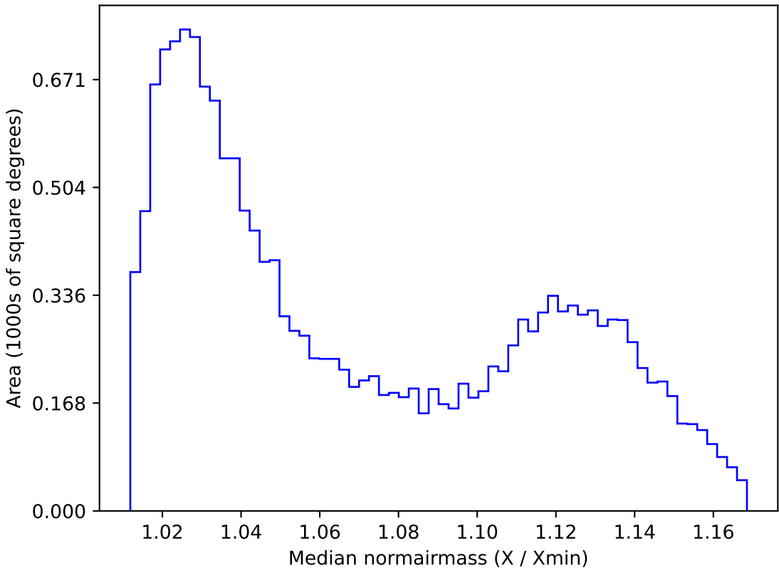
noroll_mjdp365_v3.4_10yrs WFD g band: Median normairmass
