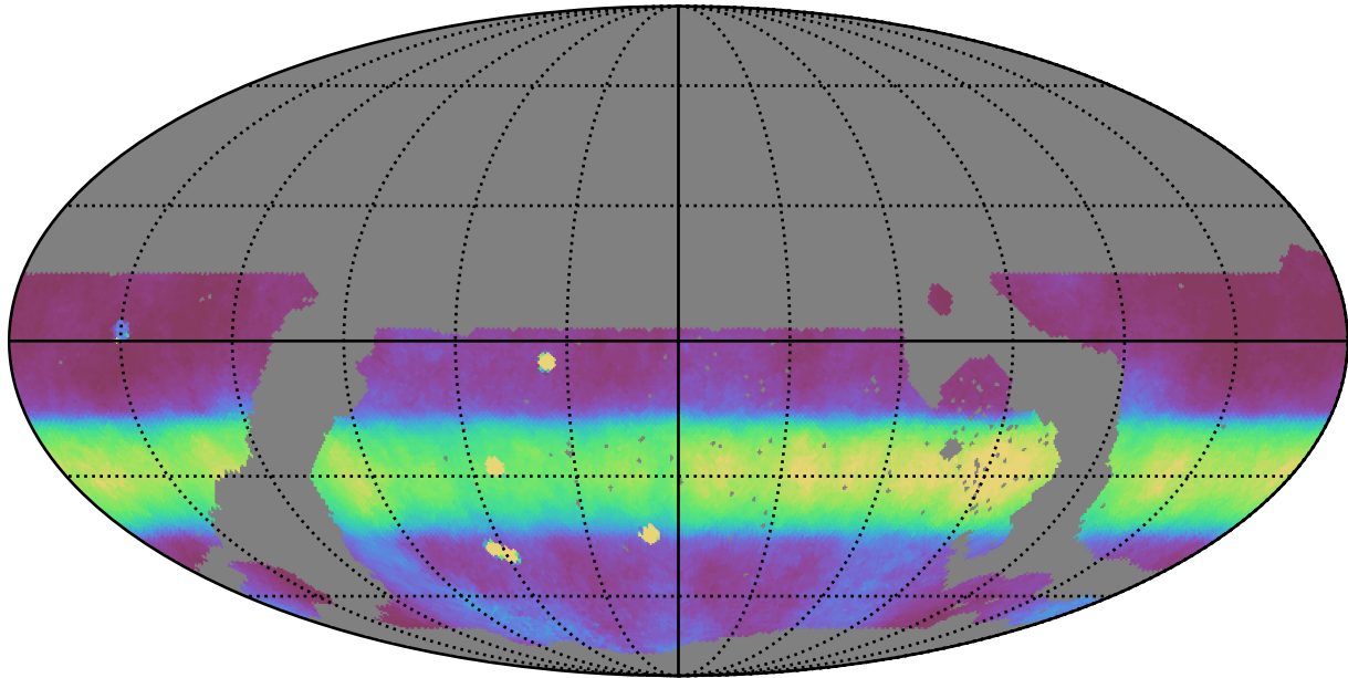
noroll_mjdp365_v3.4_10yrs WFD all bands: Median normairmass
