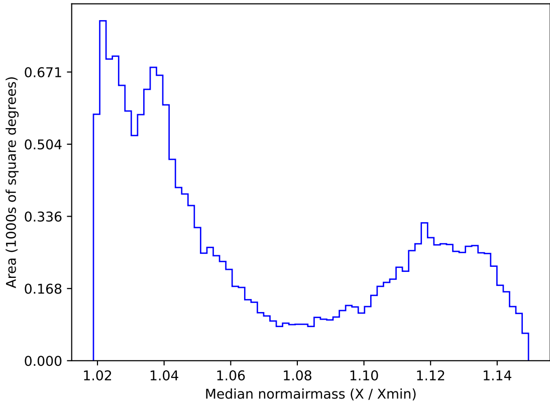
noroll_mjdp365_v3.4_10yrs WFD all bands: Median normairmass
