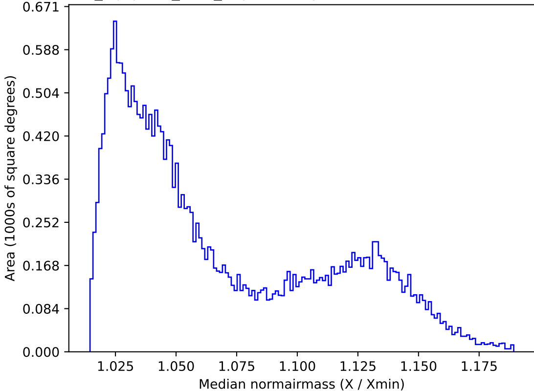
noroll_mjdp365_v3.4_10yrs All sky z band: Median normairmass
