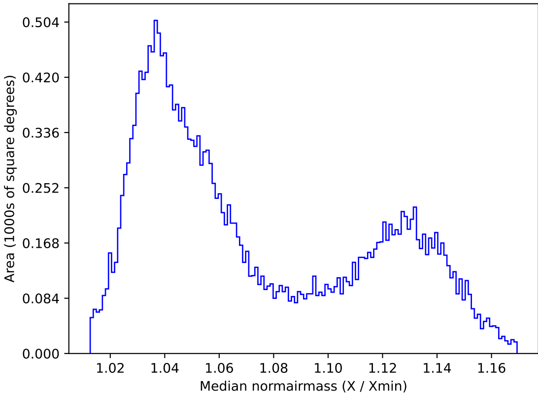
noroll_mjdp365_v3.4_10yrs All sky y band: Median normairmass
