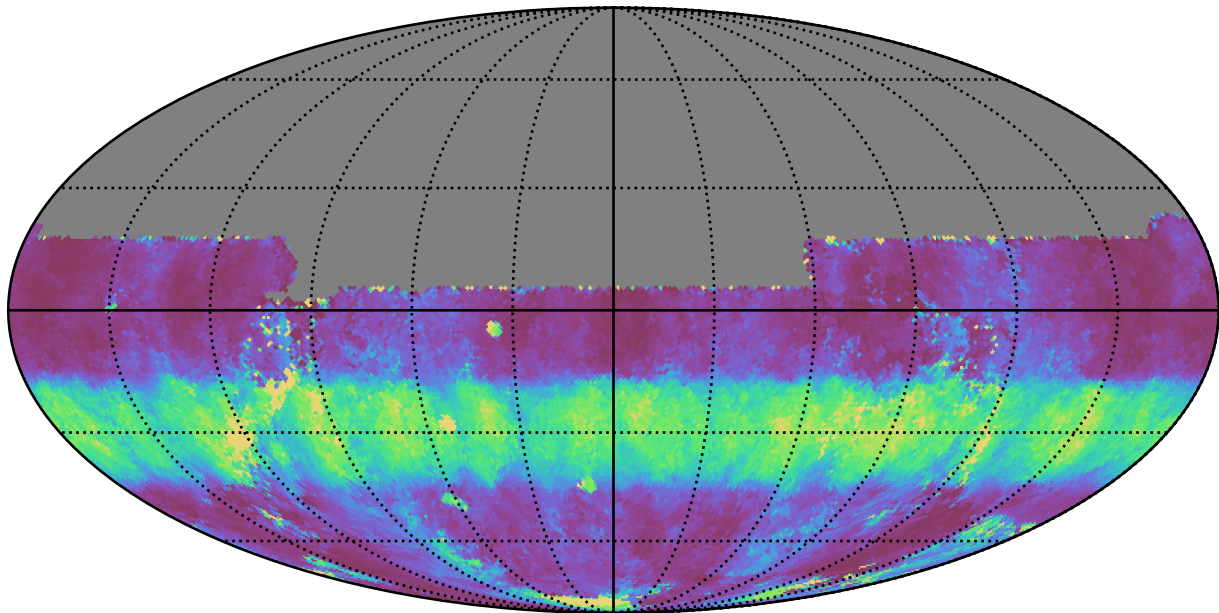
noroll_mjdp365_v3.4_10yrs All sky u band: Median normairmass
