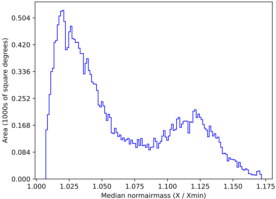
noroll_mjdp365_v3.4_10yrs All sky u band: Median normairmass
