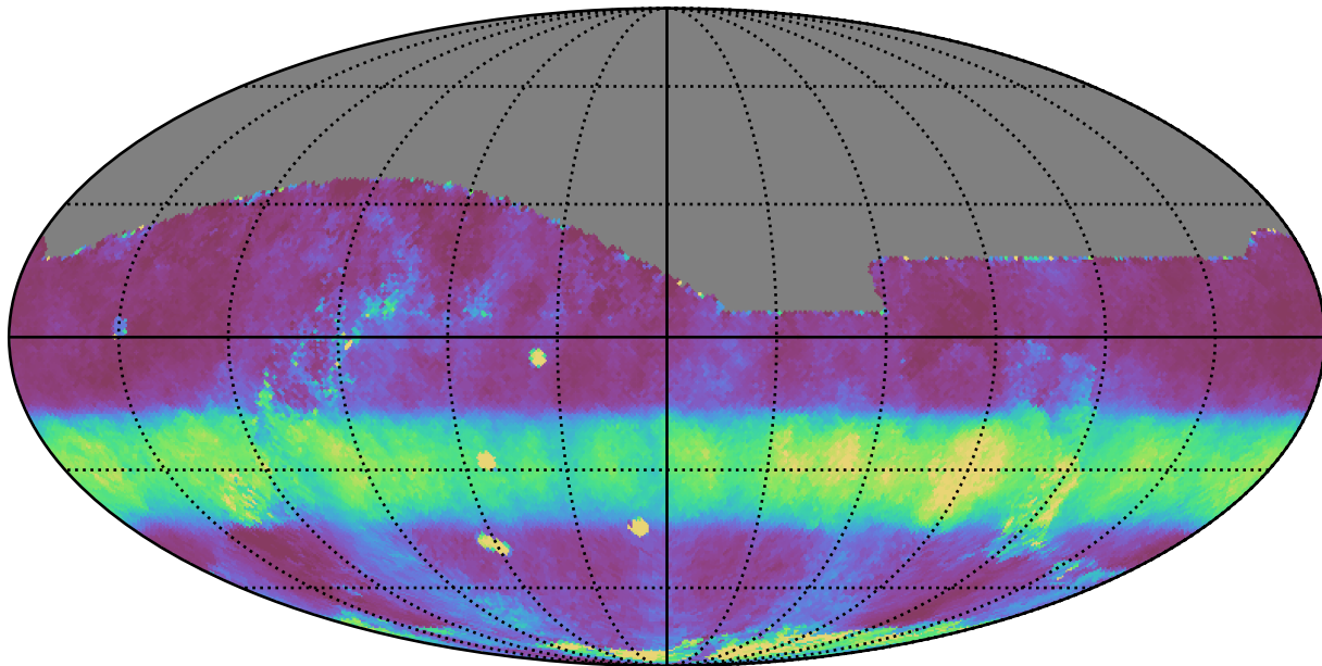
noroll_mjdp365_v3.4_10yrs All sky r band: Median normairmass
