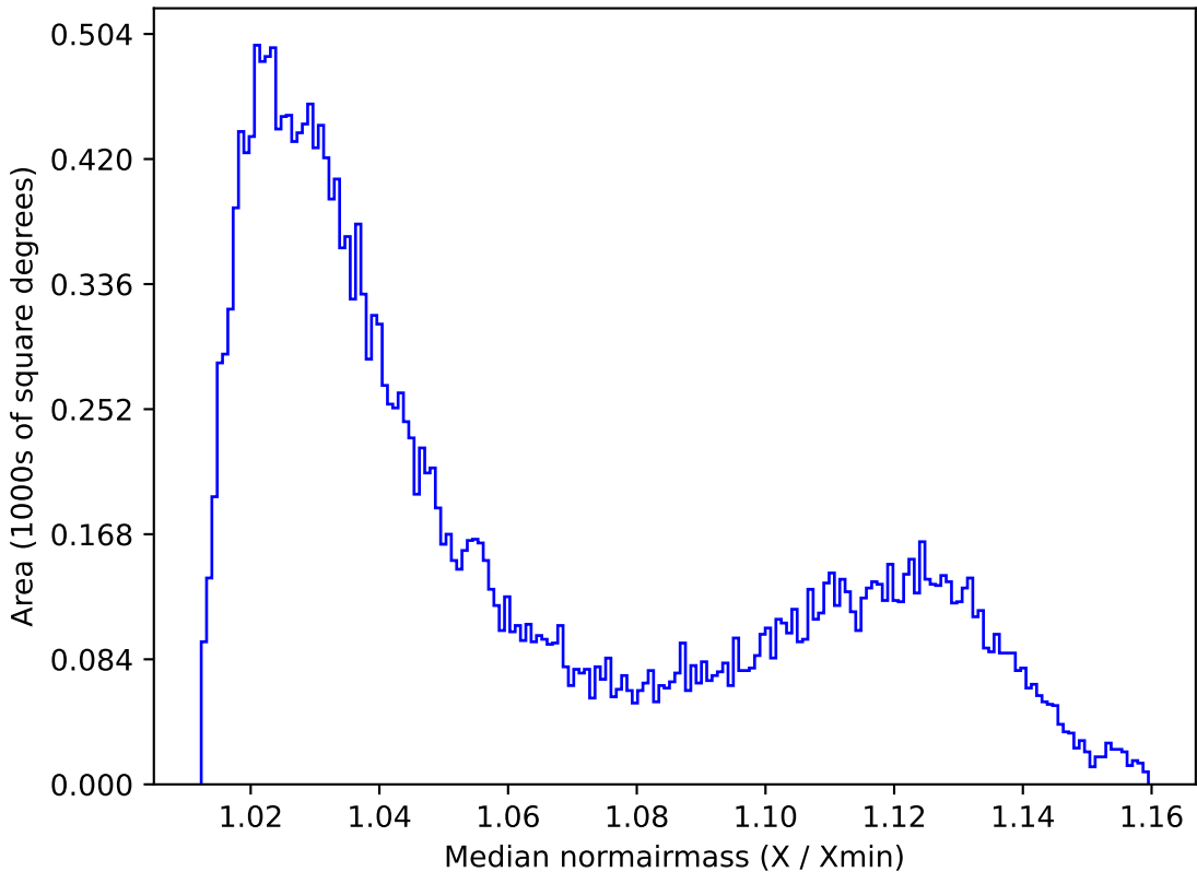
noroll_mjdp365_v3.4_10yrs All sky i band: Median normairmass
