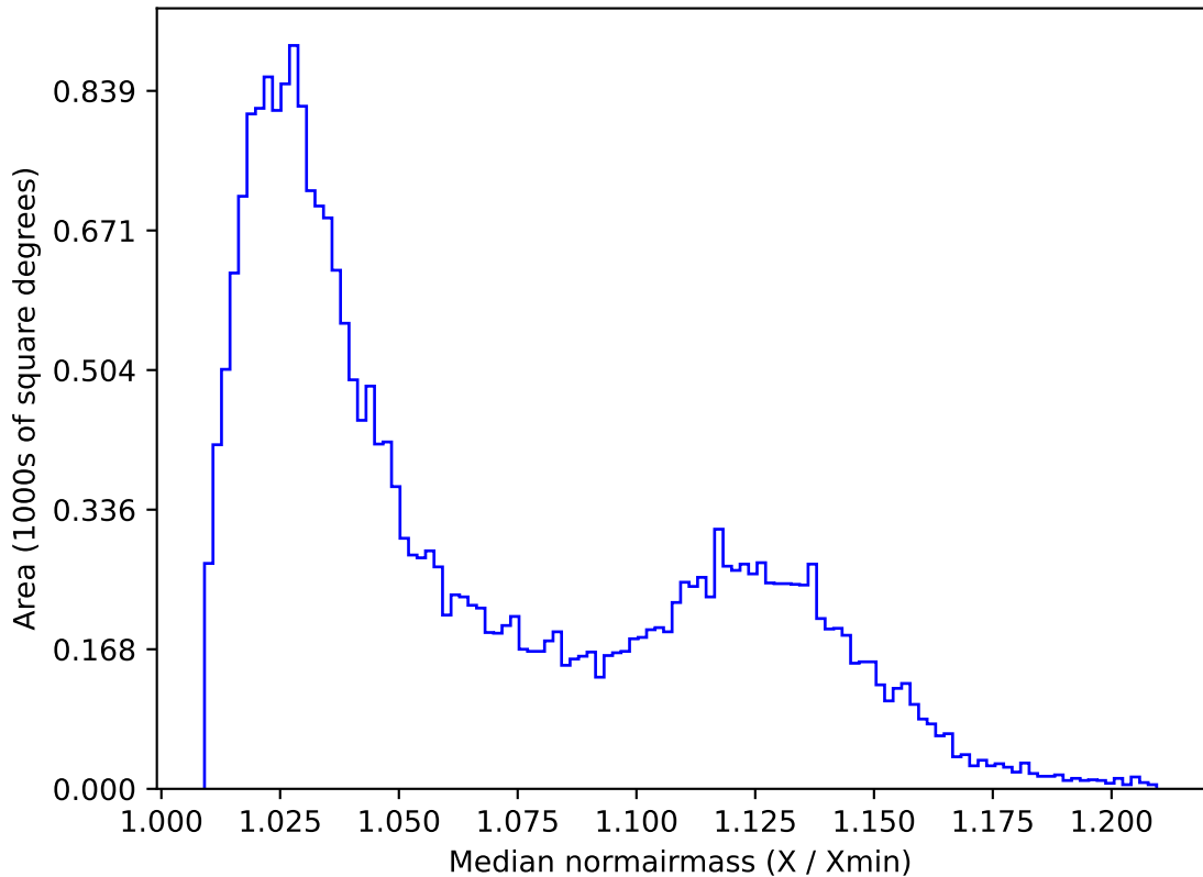
noroll_mjdp365_v3.4_10yrs All sky g band: Median normairmass
