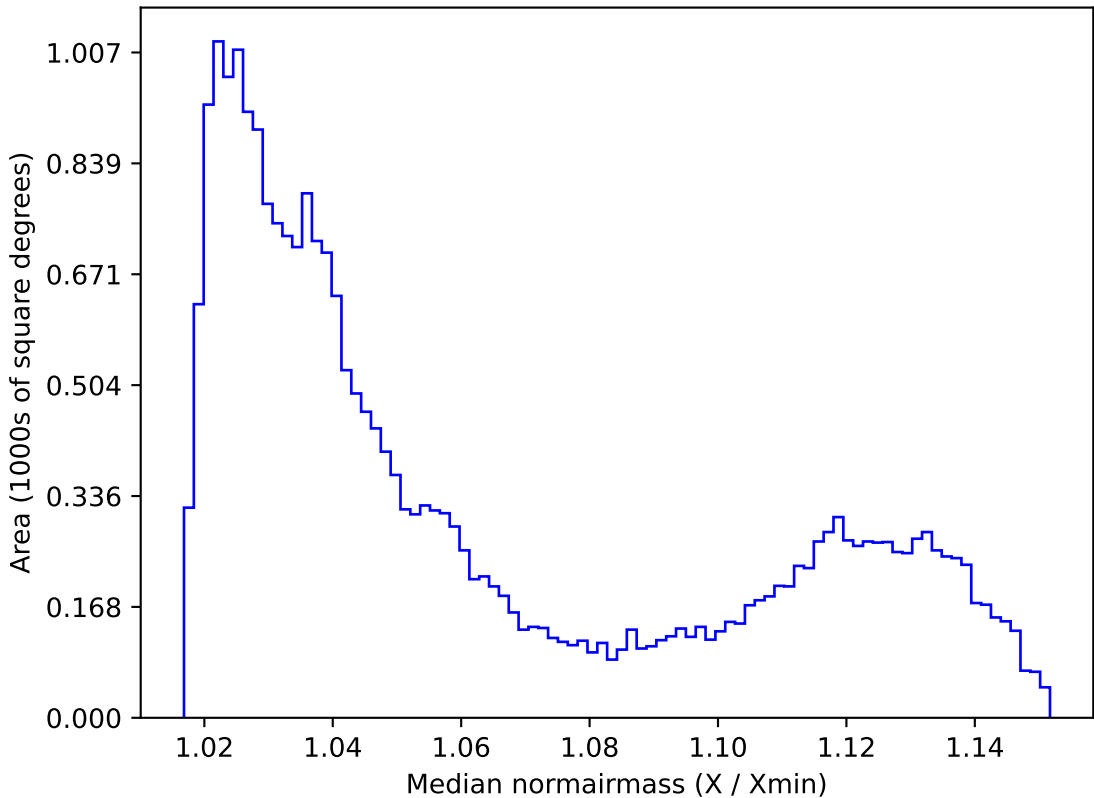
noroll_mjdp365_v3.4_10yrs All sky all bands: Median normairmass
