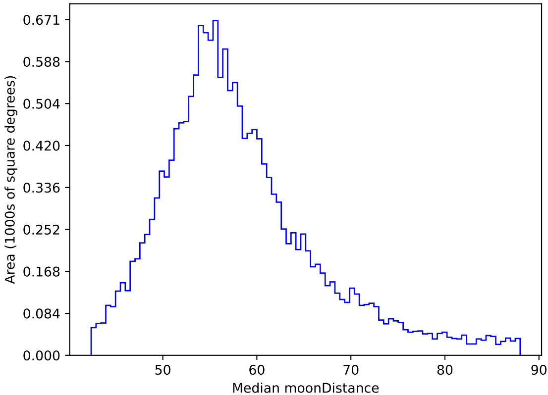
noroll_mjdp365_v3.4_10yrs WFD y band: Median moonDistance
