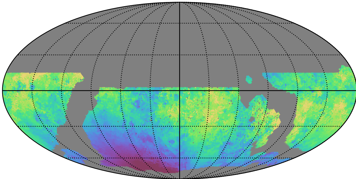
noroll_mjdp365_v3.4_10yrs WFD u band: Median moonDistance
