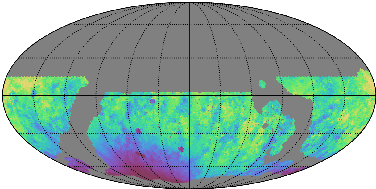
noroll_mjdp365_v3.4_10yrs WFD r band: Median moonDistance
