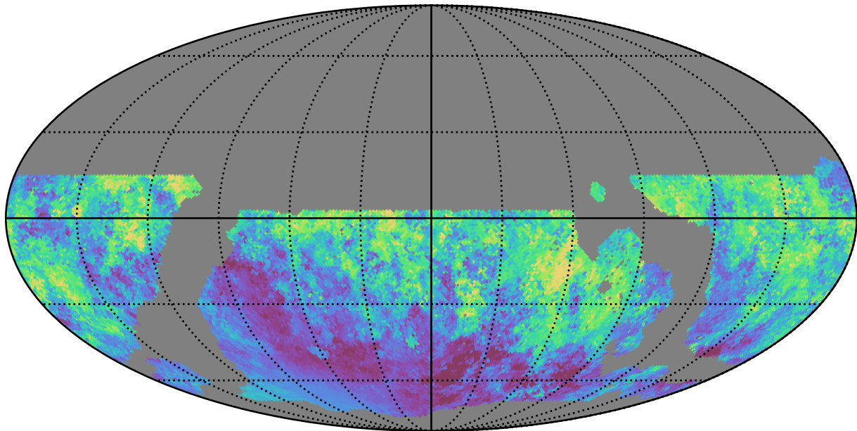
noroll_mjdp365_v3.4_10yrs WFD i band: Median moonDistance
