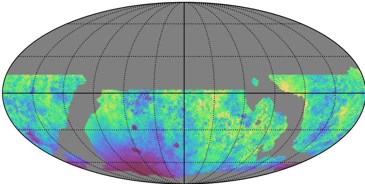
noroll_mjdp365_v3.4_10yrs WFD g band: Median moonDistance
