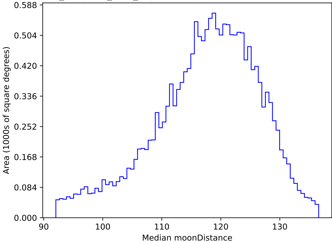
noroll_mjdp365_v3.4_10yrs WFD g band: Median moonDistance
