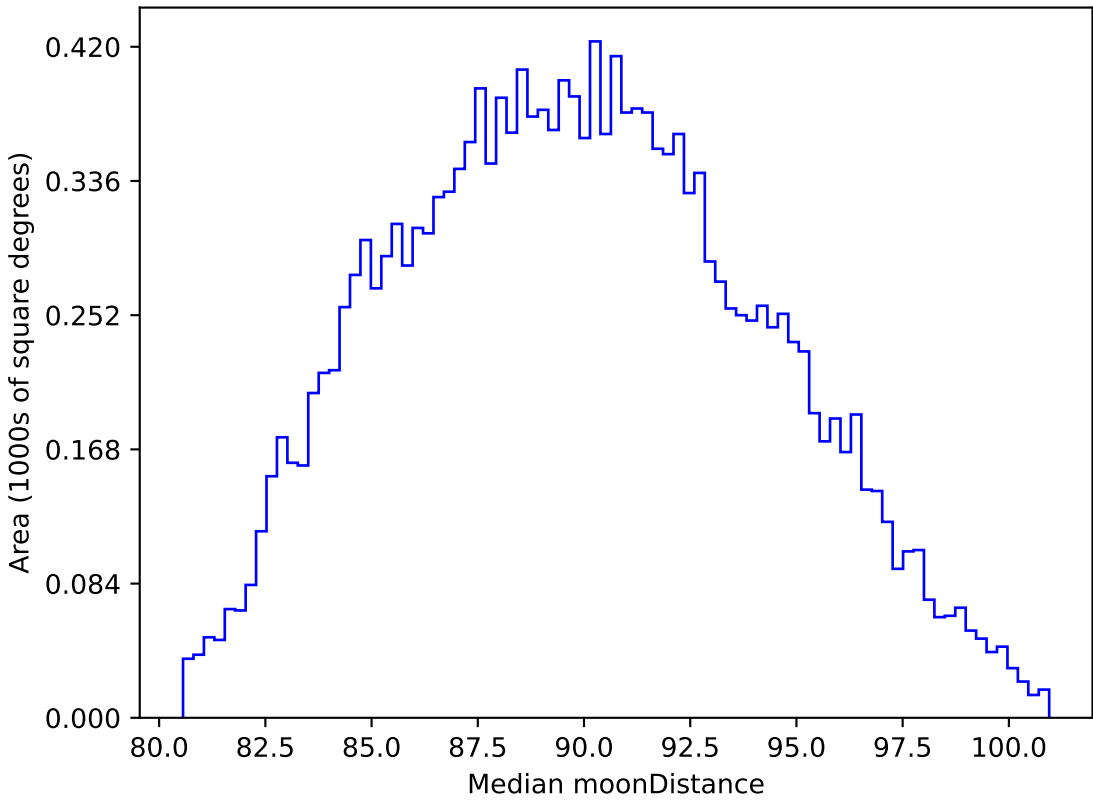
noroll_mjdp365_v3.4_10yrs WFD all bands: Median moonDistance
