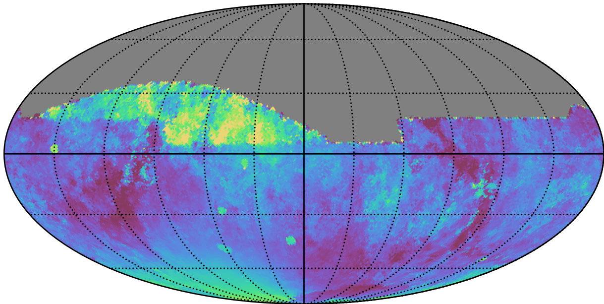
noroll_mjdp365_v3.4_10yrs All sky z band: Median moonDistance
