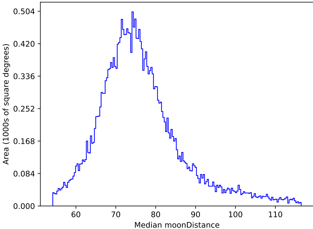
noroll_mjdp365_v3.4_10yrs All sky z band: Median moonDistance
