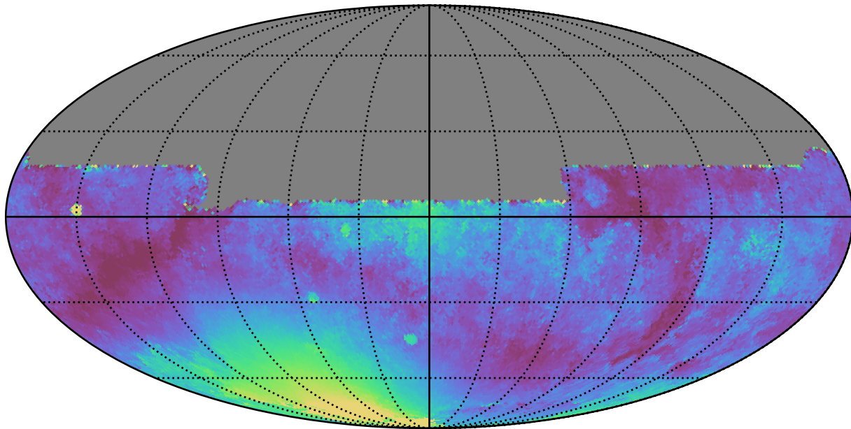
noroll_mjdp365_v3.4_10yrs All sky y band: Median moonDistance
