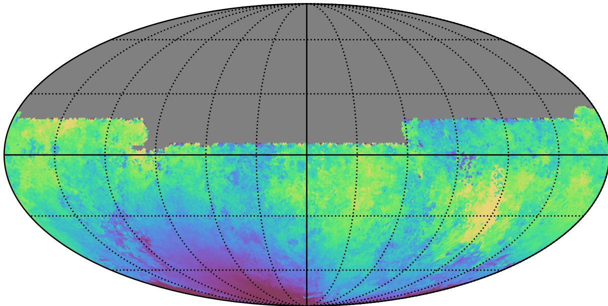
noroll_mjdp365_v3.4_10yrs All sky u band: Median moonDistance
