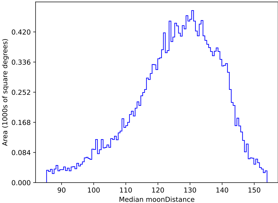
noroll_mjdp365_v3.4_10yrs All sky u band: Median moonDistance
