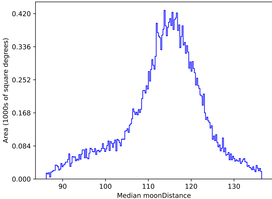
noroll_mjdp365_v3.4_10yrs All sky r band: Median moonDistance
