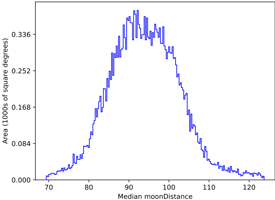
noroll_mjdp365_v3.4_10yrs All sky i band: Median moonDistance
