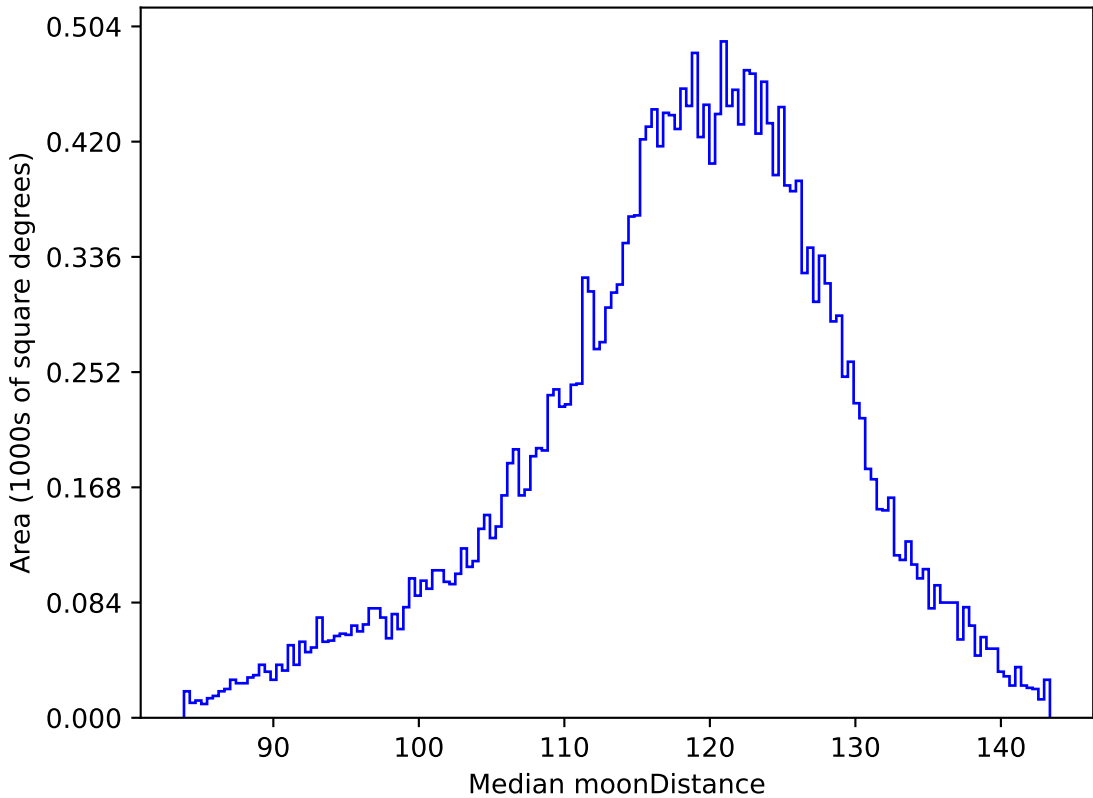
noroll_mjdp365_v3.4_10yrs All sky g band: Median moonDistance
