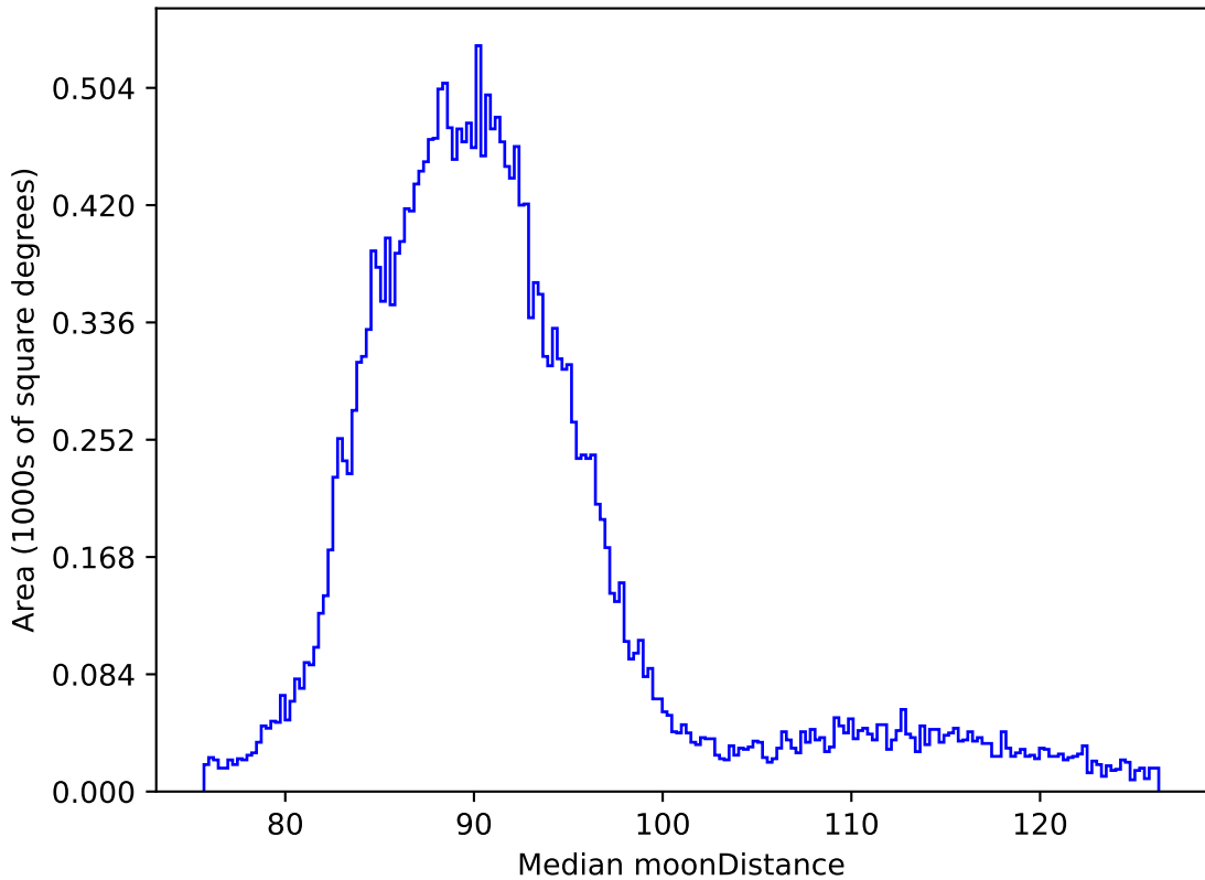
noroll_mjdp365_v3.4_10yrs All sky all bands: Median moonDistance
