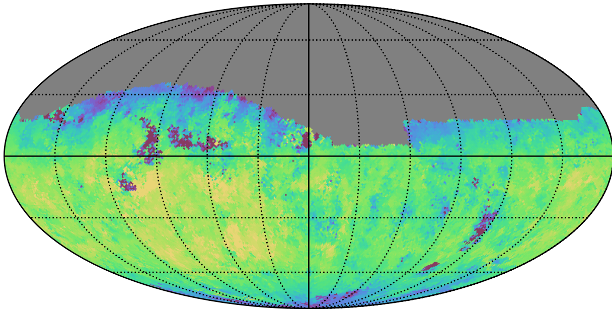
noroll_mjdp365_v3.4_10yrs Yr 1 z band: Median fiveSigmaDepth
